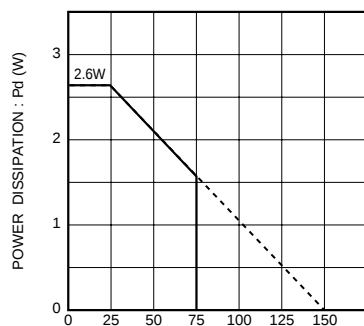
Fig.4 Power dissipation
