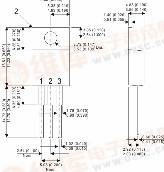
TO220-AC Package Outline. Dimensions in mm (inches)
