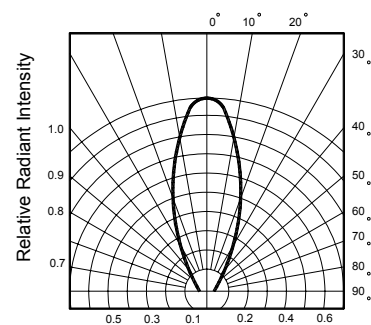
FIG.5 Radiant Diagram
