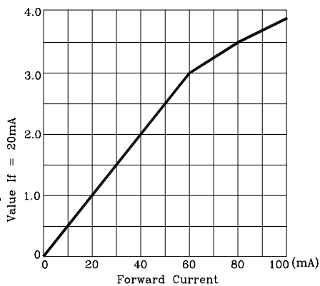
FIG.4 Relative Radiant Vs. Forward Current
