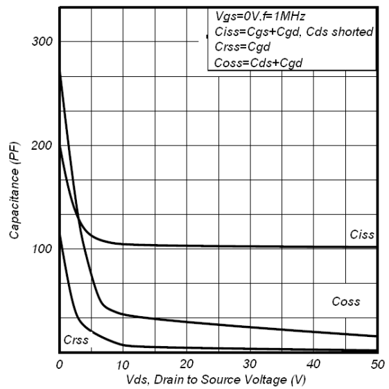
Fig 8. Capacitance Characteristics
