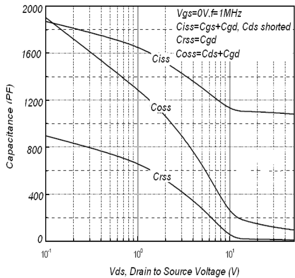
Fig 8. Capacitance Characteristics
