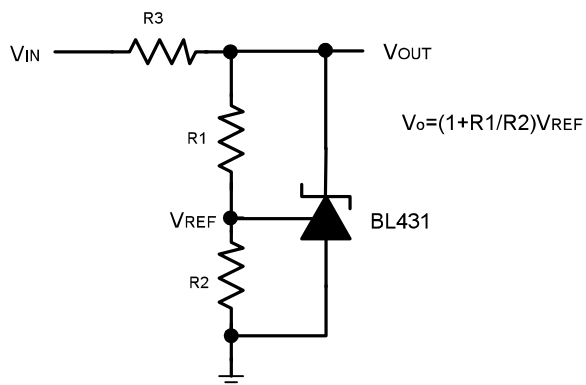
Figure 15. Shunt Regulator
