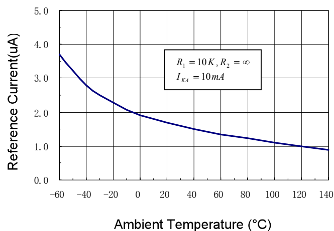
Figure 7.Reference Current vs. Ambient Temperature
