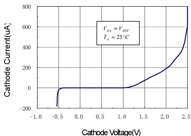
Figure 9. Current vs. Cathode Voltage
