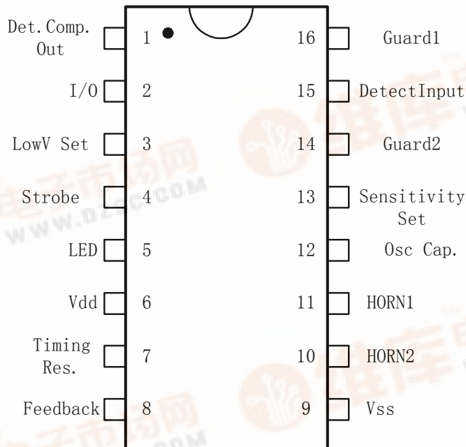
Figure 1 管脚排列
