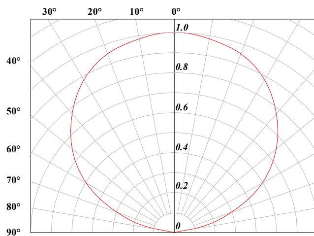
Radiation pattern.
