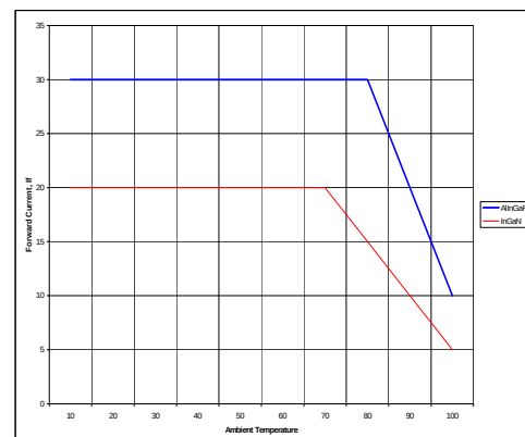
Fig. 4 Maximum forward current vs. temperature
