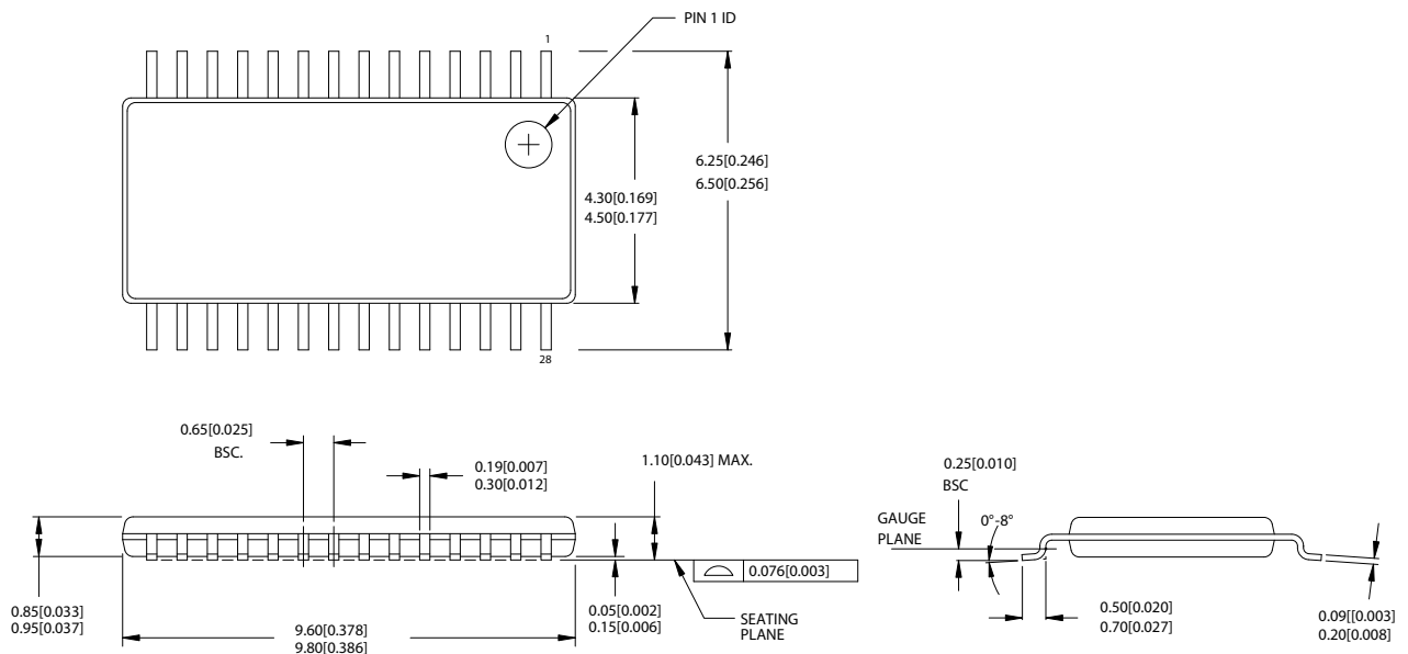
Figure 8. 28-Pin Thin Shrink Small Outline Package (4.40-mm Body) ZZ28
