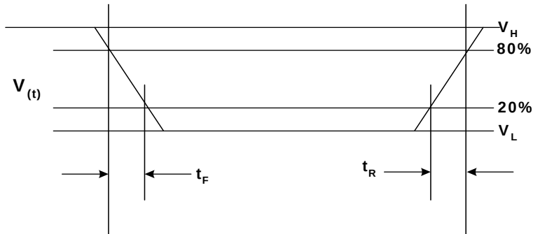
Figure 4. Input and Output Waveforms
