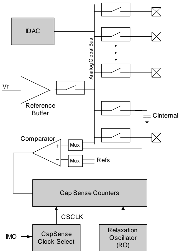
Analog System Block Diagram
