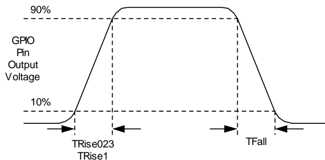
Figure 2-2. GPIO Timing Diagram
