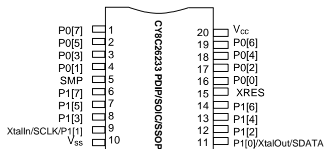
Figure 3: CY8C26233
