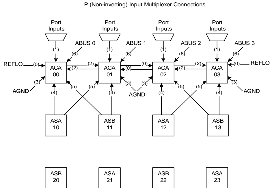
Figure 19: PMux Connections
