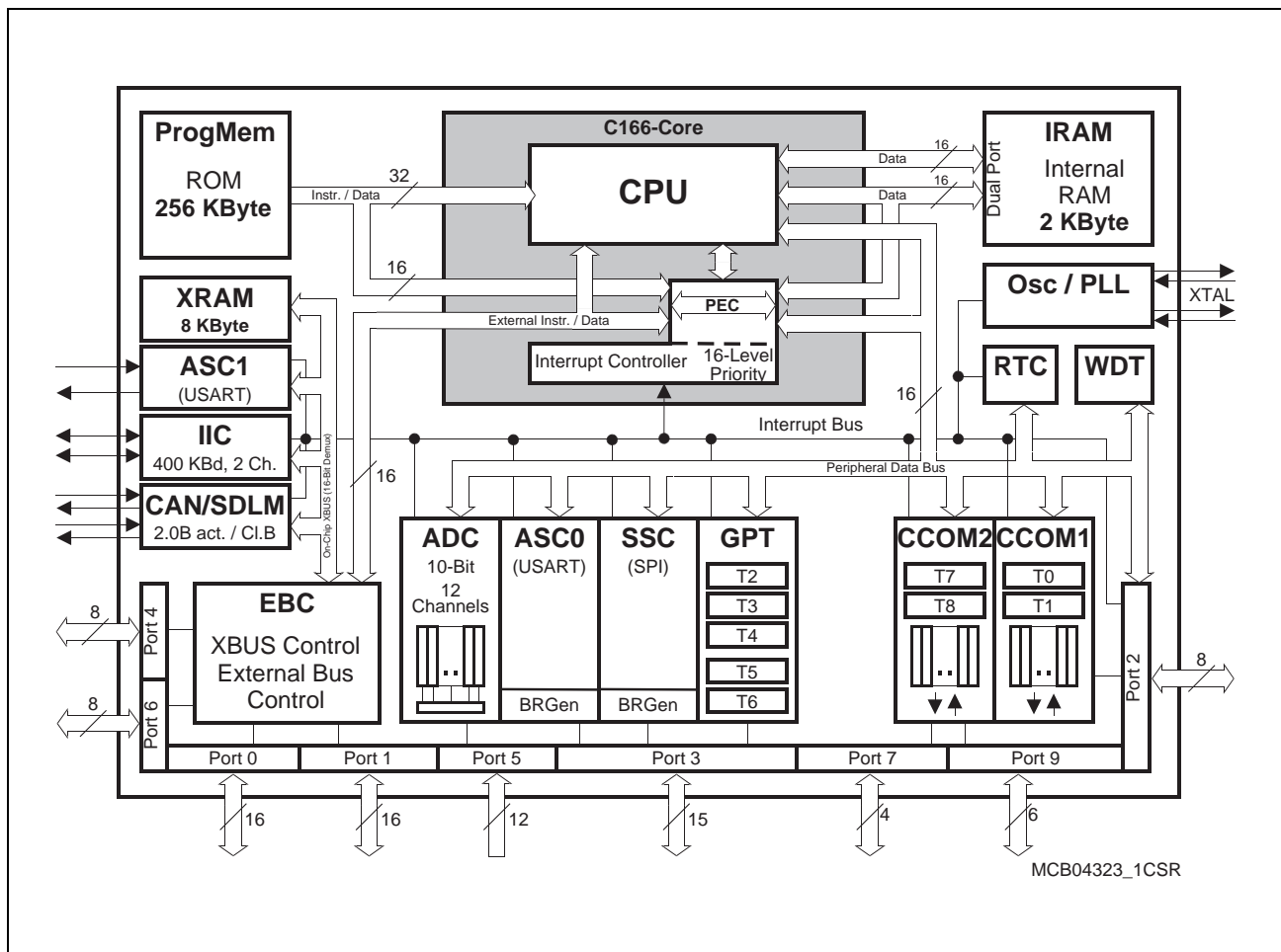
Figure 3 Block Diagram
