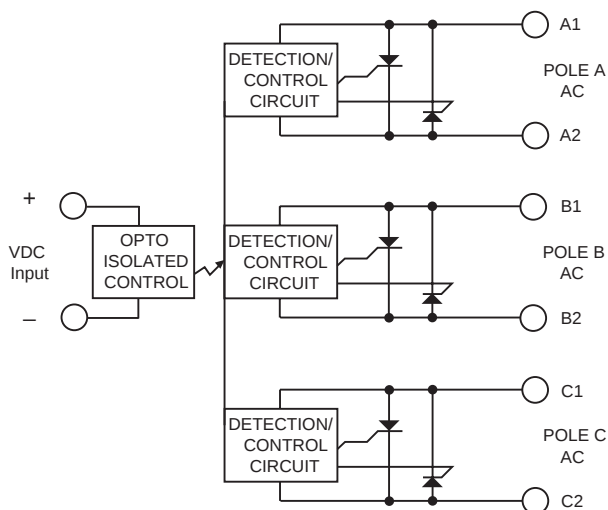
Figure 3 — Block Diagram
