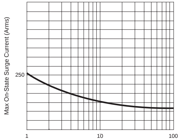
Figure 4 — Surge Current Curves
