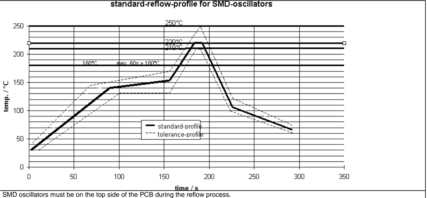
standard-reflow-profile for SMD-oscillators
