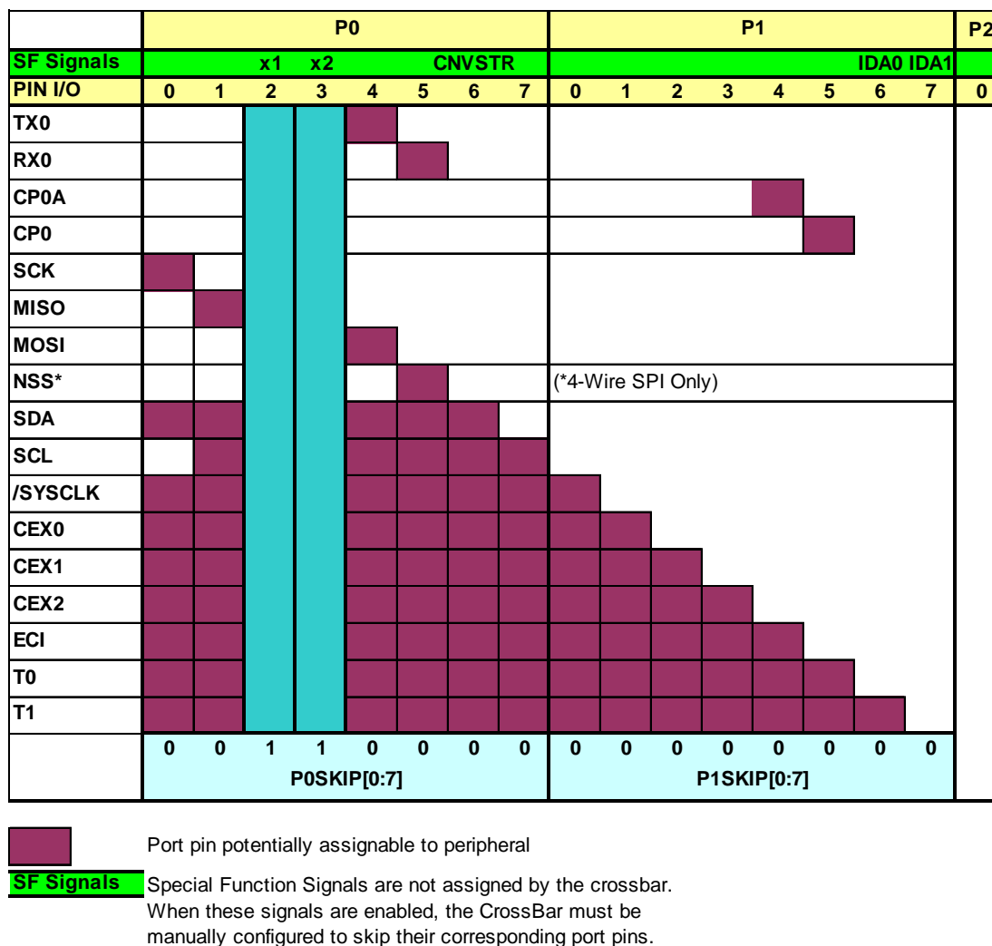
Figure 18.4. Crossbar Priority Decoder with Crystal Pins Skipped
