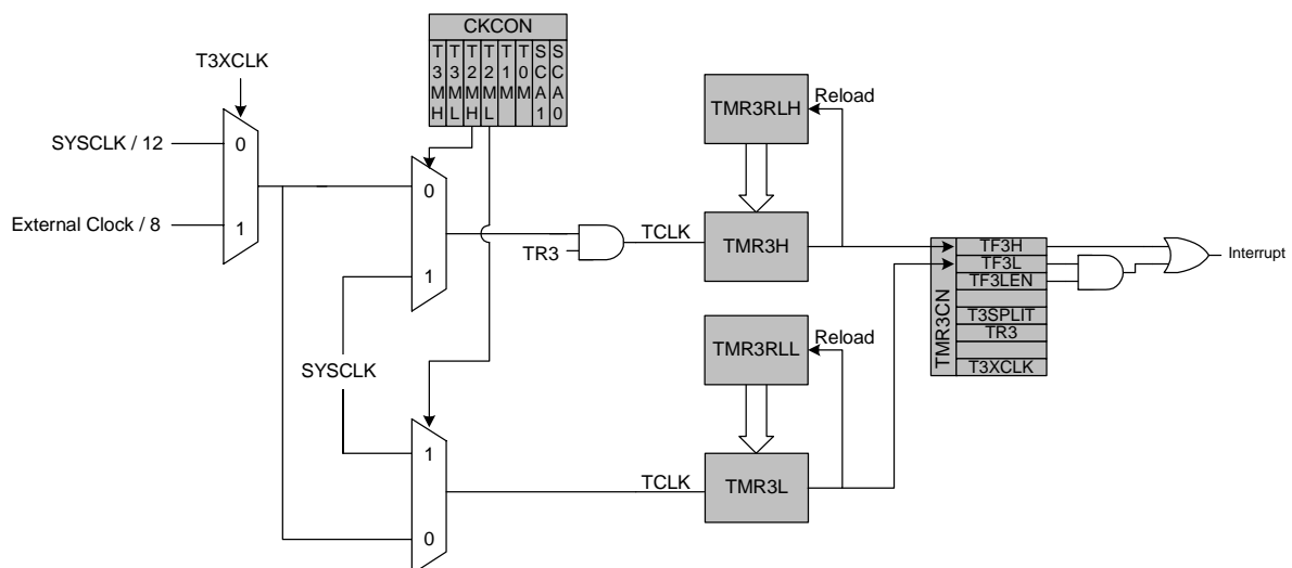
Figure 22.7. Timer 3 8-Bit Mode Block Diagram
