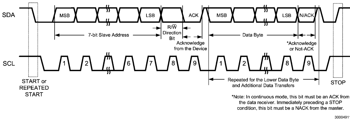
FIGURE 4. Basic Operation.
