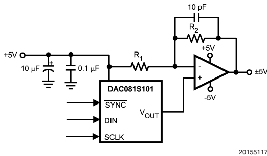
FIGURE 13. Bipolar Operation
