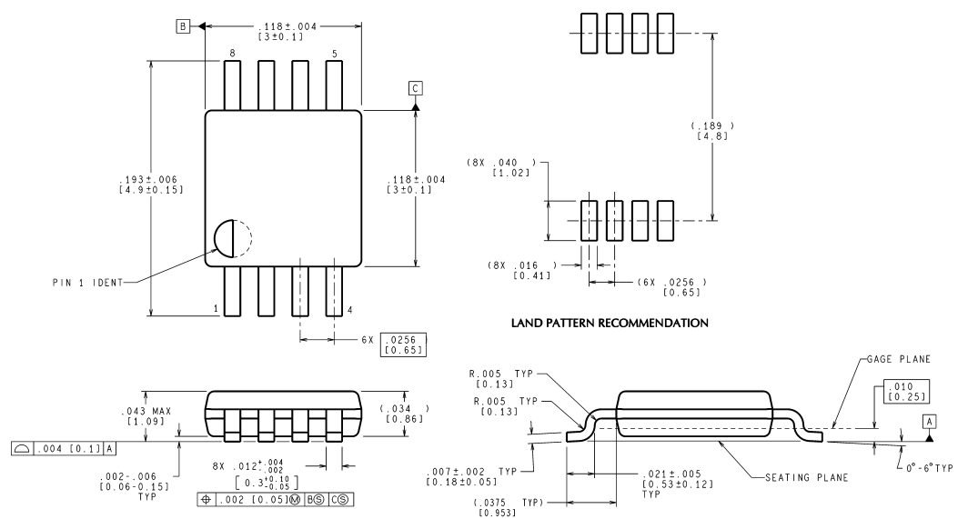
8-Lead MSOP Order Numbers DAC081S101C1MM NS Package Number MUA08A
