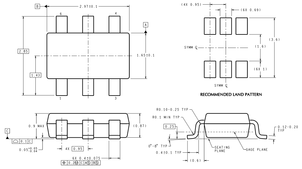
6-Lead TSOT Order Numbers DAC081S101CIMK NS Package Number MK06A
