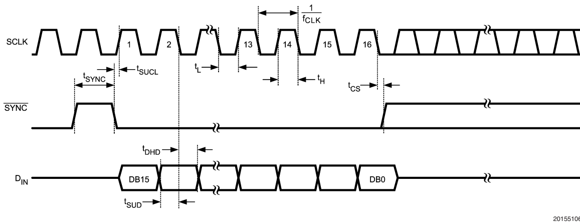
FIGURE 2. DAC081S101 Timing
