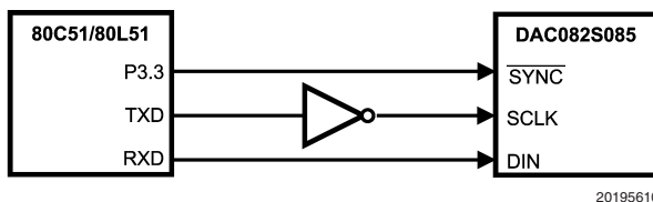
FIGURE 11. 80C51/80L51 Interface
