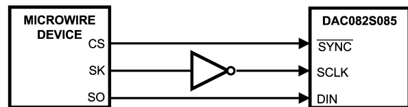
FIGURE 13. Microwire Interface
