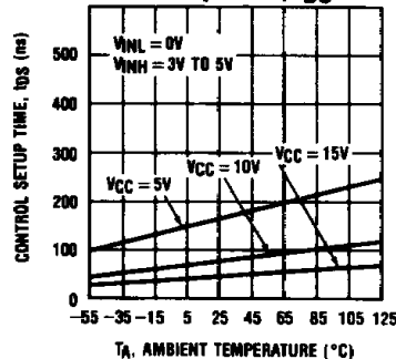
Data Setup Time, t_{DS}
