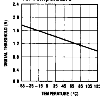
Digital Input Threshold vs. Temperature
