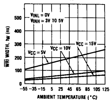
Write Width, t_w
