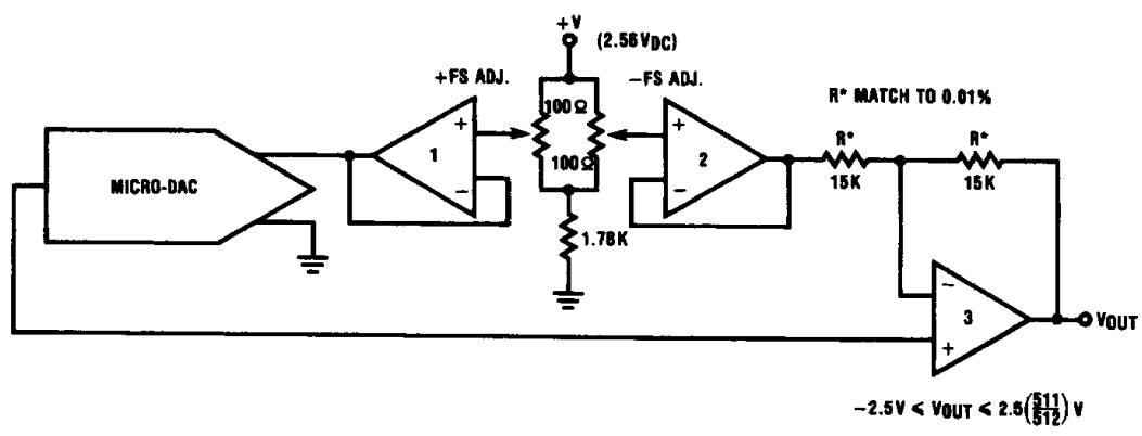
FIGURE 14. Voltage Switching with a Bipolar Output Voltage
