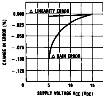
Errors vs. Supply Voltage
