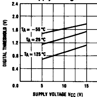
Digital Threshold vs. Supply Voltage
