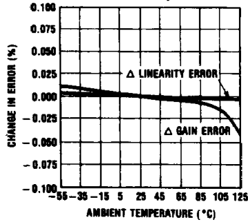
Errors vs. Temperature
