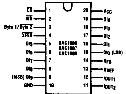
DAC1006/1007/1008 (20-Pin Parts) Dual-In-Line Package
