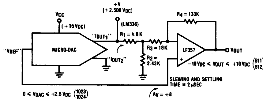
FIGURE 11. Increasing the Output Voltage Swing
