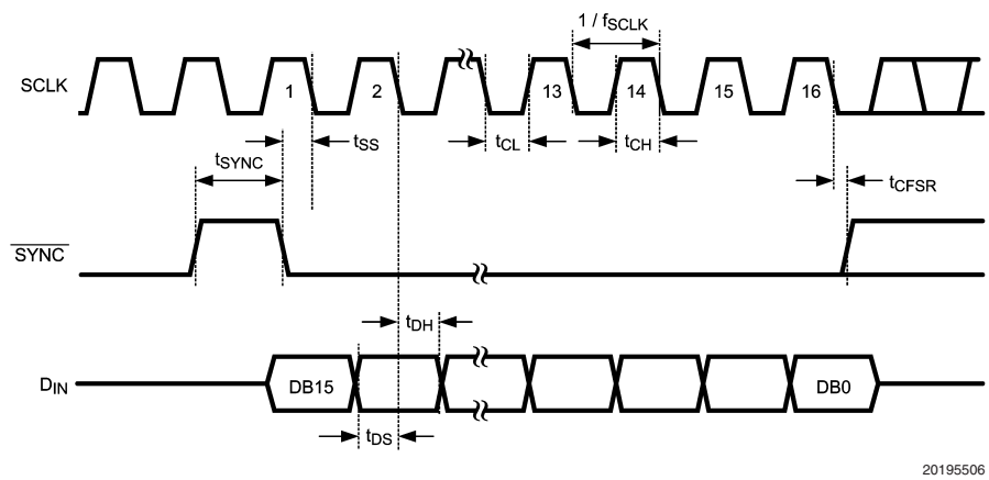
FIGURE 2. Serial Timing Diagram
