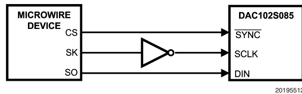
FIGURE 13. Microwire Interface
