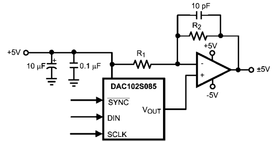
FIGURE 9. Bipolar Operation
