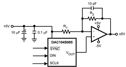
FIGURE 9. Bipolar Operation
