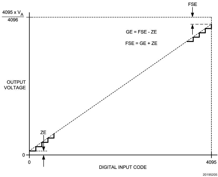
FIGURE 1. Input / Output Transfer Characteristic
