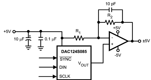
FIGURE 9. Bipolar Operation
