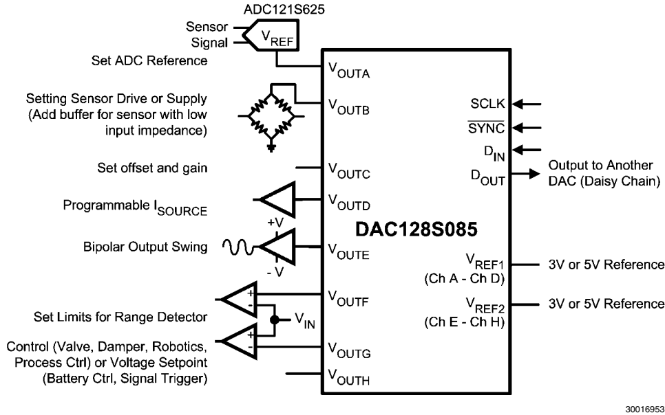
FIGURE 14. Industrial Application
