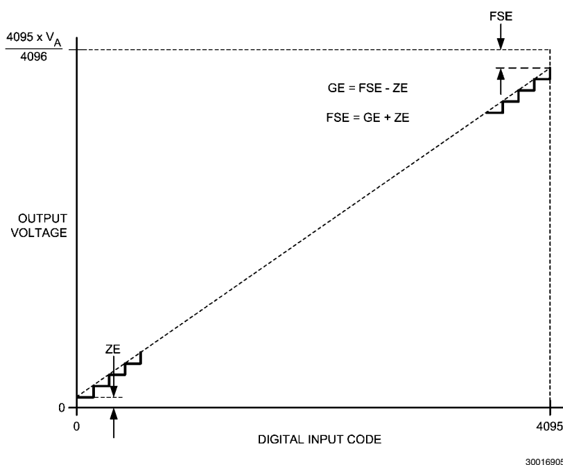
FIGURE 2. Input / Output Transfer Characteristic
