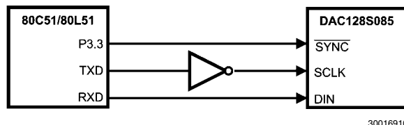
FIGURE 18. 80C51/80L51 Interface
