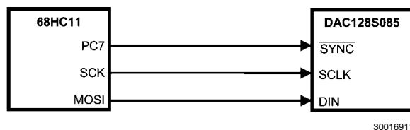
FIGURE 19. 68HC11 Interface
