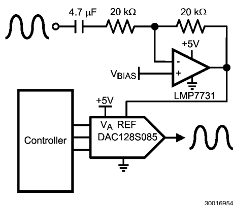
FIGURE 16. Programmable Attenuator
