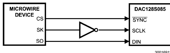
FIGURE 20. Microwire Interface
