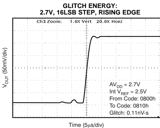
Time (5µs/div) Figure 88.
