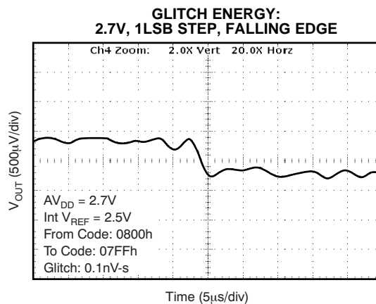
Time (5µs/div) Figure 85.
