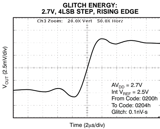
Time (2µs/div) Figure 86.
