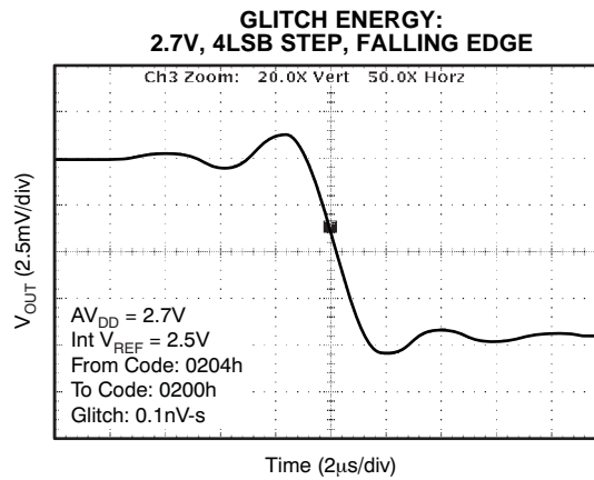
Time (2µs/div) Figure 87.
