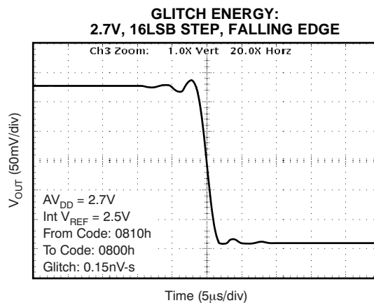
Time (5µs/div) Figure 89.
