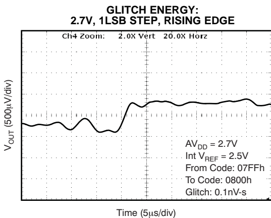
Time (5µs/div) Figure 84.
