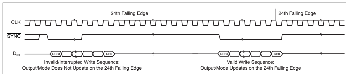
Figure 95. \overline{\text{SYNC}} Interrupt Facility
