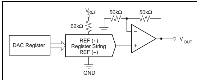
Figure 41. DAC8552 Architecture
