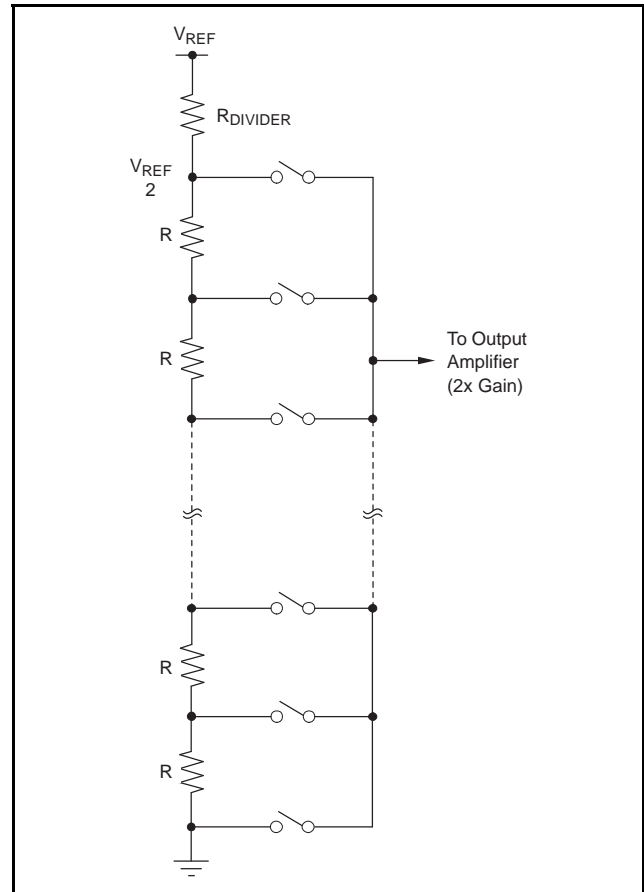
Figure 42. Resistor String
