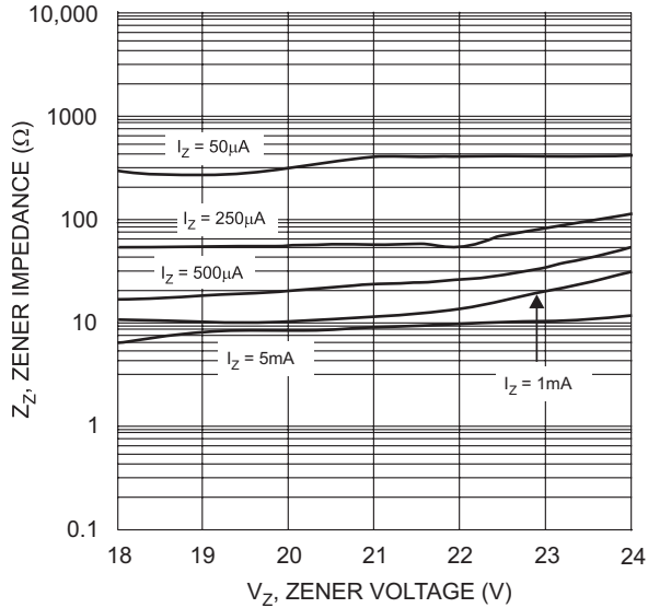
Fig. 12 Typical Zener Impedance Characteristics, DDZ18C - DDZ24C
