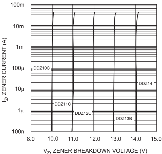
Fig. 5 Typical Reverse Characteristics, DDZ10C - DDZ14
