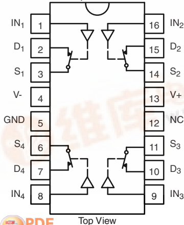
Dual-In-Line, SOIC and TSSOP
