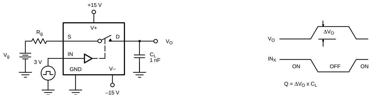
FIGURE 4. Charge Injection
