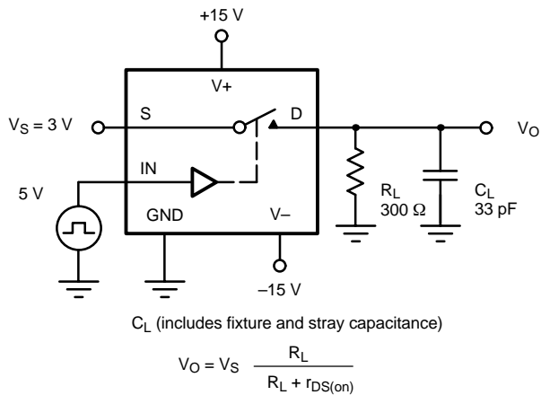
FIGURE 2. Switching Time
