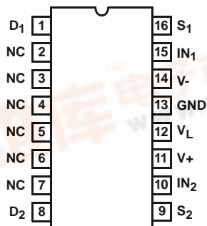
DG401 (16 LD SOIC, TSSOP) TOP VIEW
