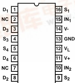
DG403 (16 LD SOIC, TSSOP) TOP VIEW
