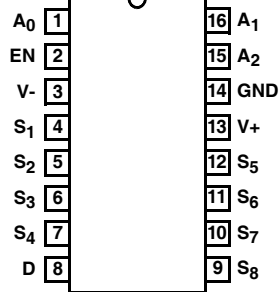
DG408 (PDIP, SOIC, TSSOP) TOP VIEW
