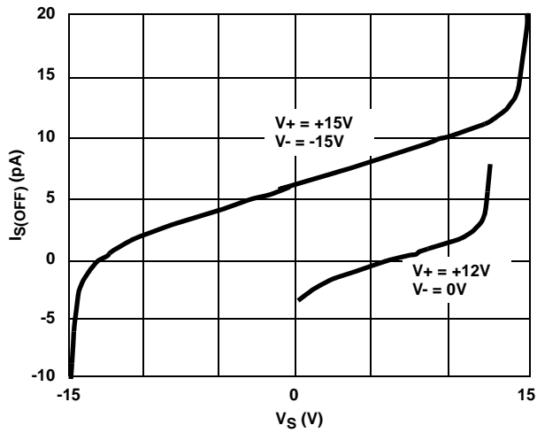
FIGURE 16. SOURCE LEAKAGE CURRENT vs SOURCE VOLTAGE
