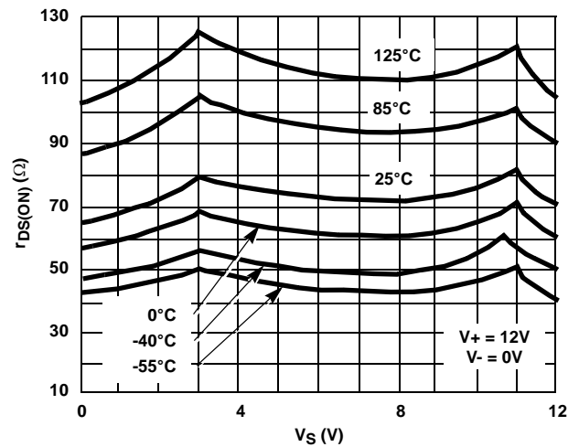
FIGURE 27. r_{DS(ON)} vs V_S AND TEMPERATURE (SINGLE SUPPLY)
