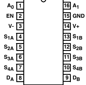
DG409 (PDIP, SOIC, TSSOP) TOP VIEW
