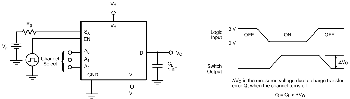
FIGURE 5. Charge Injection
