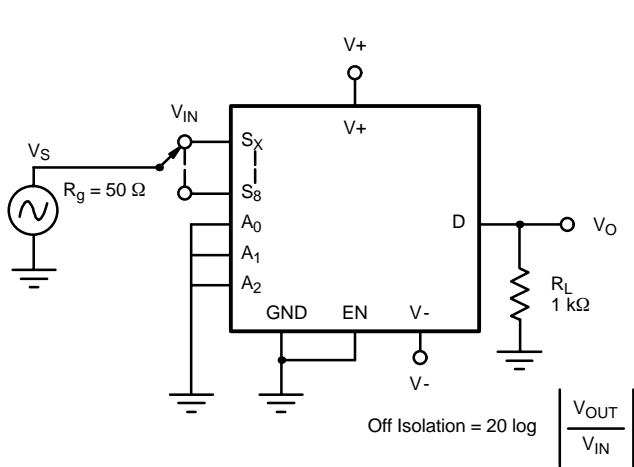
FIGURE 6. Off Isolation
