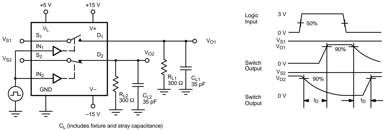
FIGURE 3. Break-Before-Make (DG413)
