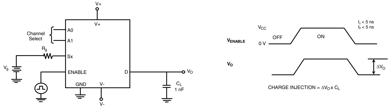
Figure 4. Charge Injection
