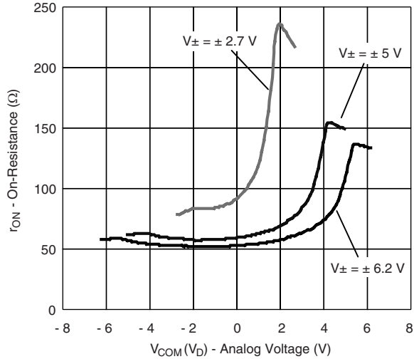
On-Resistance vs. V_D (Dual Supply)
