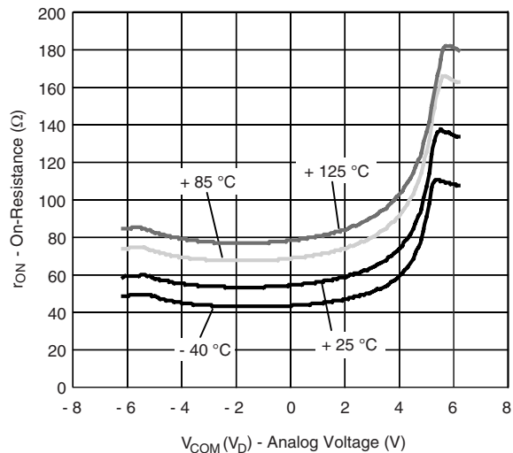
On-Resistance vs. Temperature (Dual Supply)
