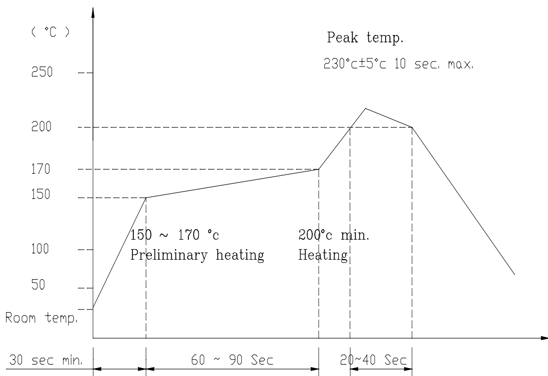
Figure 5. REFLOW PROFILE
