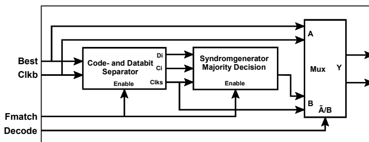
Fig.5: Decoder
