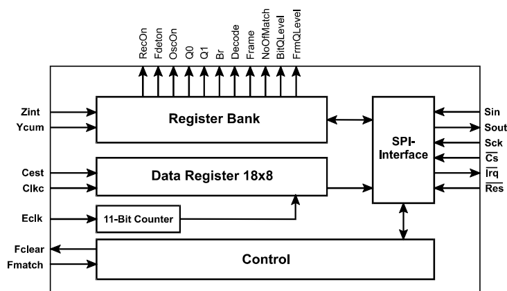
Fig.7: Interface
