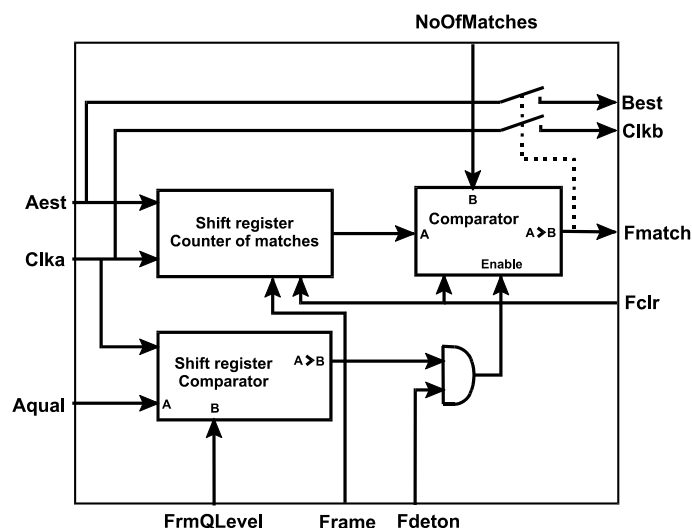
Fig.4: Frame Detector
