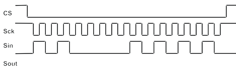
Fig. 8: Write Sequence
