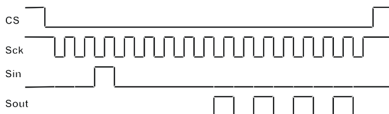
Fig. 9: Read Sequence
