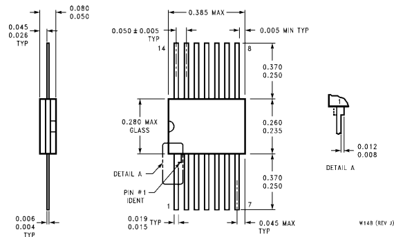
14-Lead Ceramic Flat Package (W) Order Number 5432FMB or DM5432W NS Package Number W148
