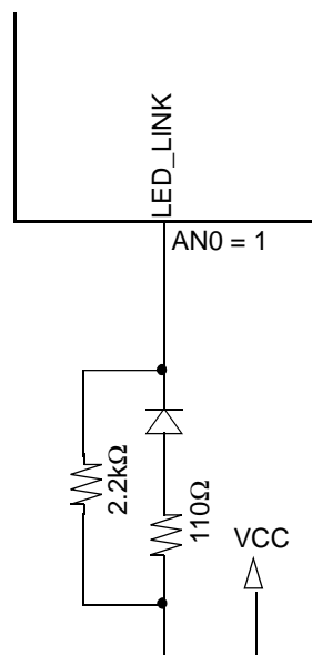
Figure 3. AN0 Strapping and LED Loading Example
