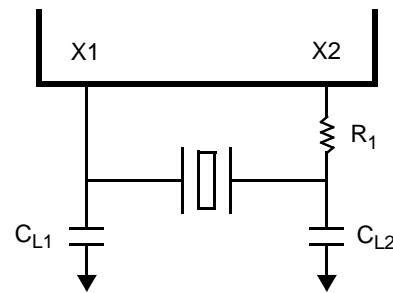
Figure 14. Crystal Oscillator Circuit
