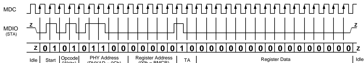
Figure 12. Typical MDC/MDIO Write Operation
