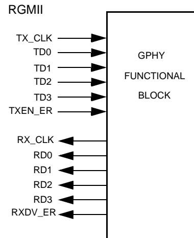
Figure 5. RGMII Signals
