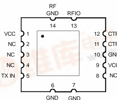
DR4101 Pin Out
