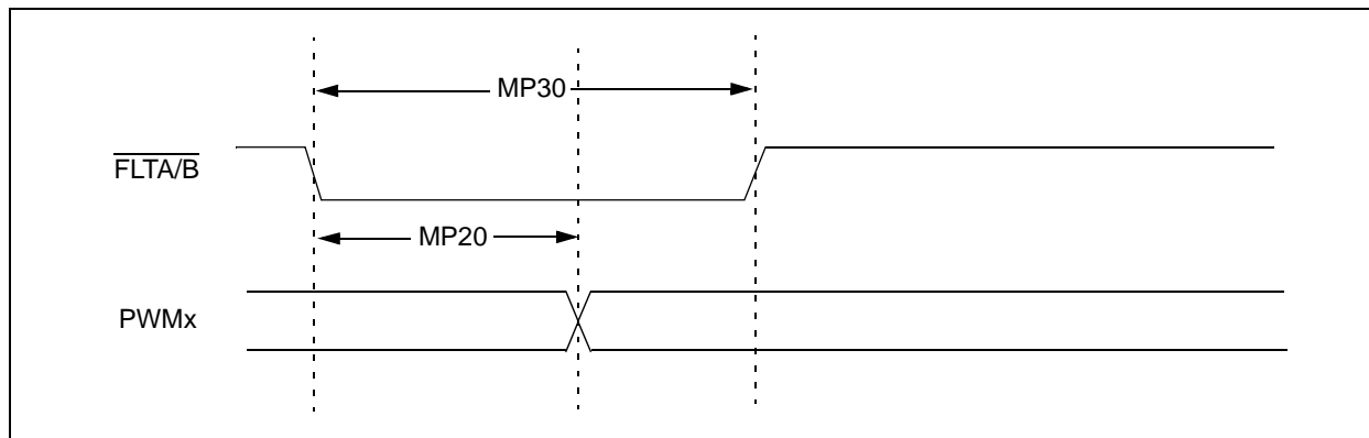
FIGURE 21-10: SMPS PWM MODULE FAULT TIMING CHARACTERISTICS
