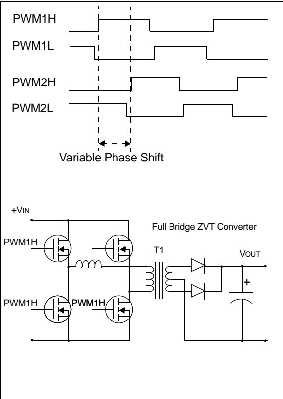
FIGURE 12-24: APPLICATION OF VARIABLE PHASE PWM MODE
