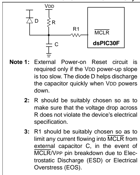
FIGURE 18-10: EXTERNAL POWER-ON RESET CIRCUIT (FOR SLOW V_{DD} POWER-UP)
