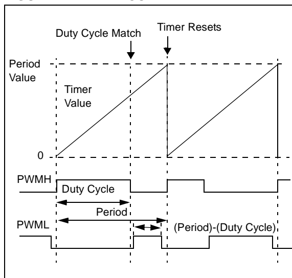
FIGURE 12-4: COMPLEMENTARY PWM
