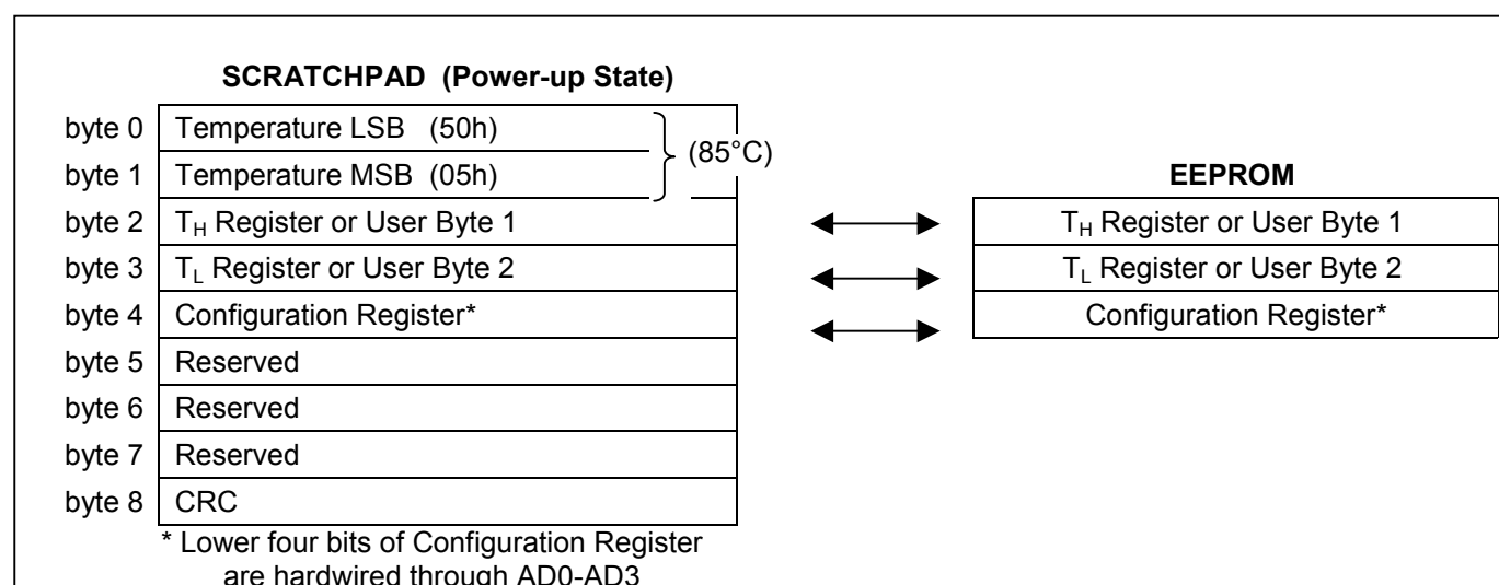
Figure 7. DS1825 MEMORY MAP
