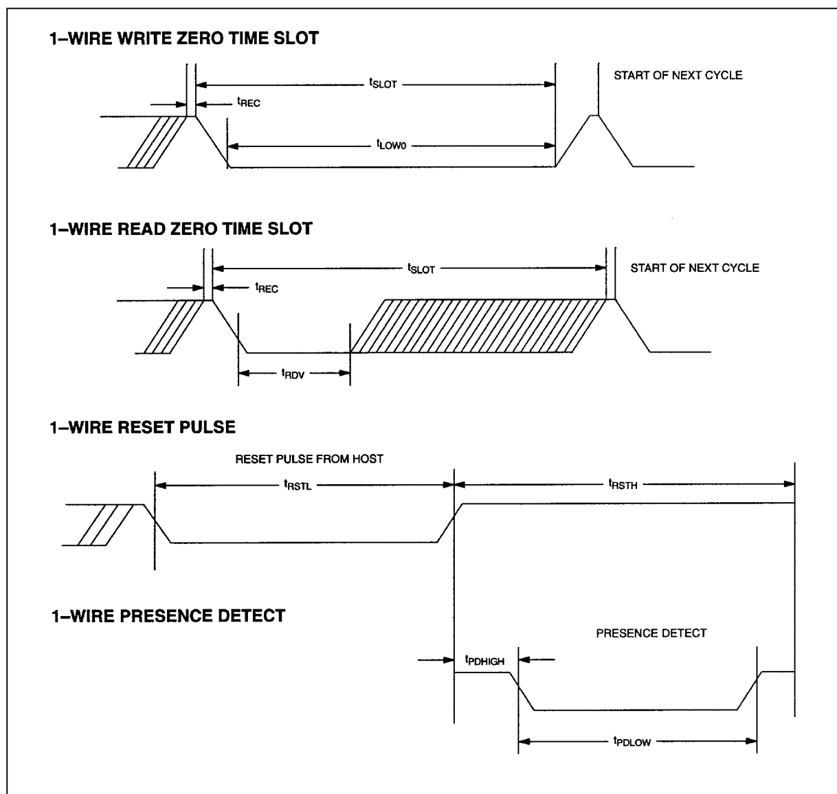
Figure 19. TIMING DIAGRAMS
