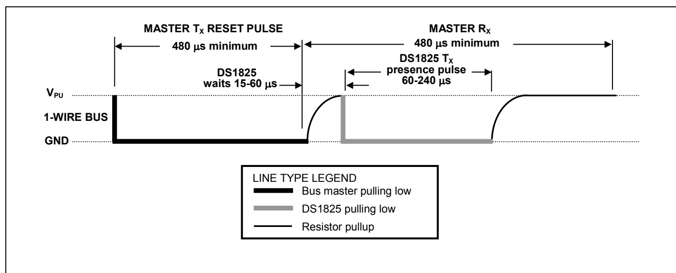
Figure 14. INITIALIZATION TIMING
