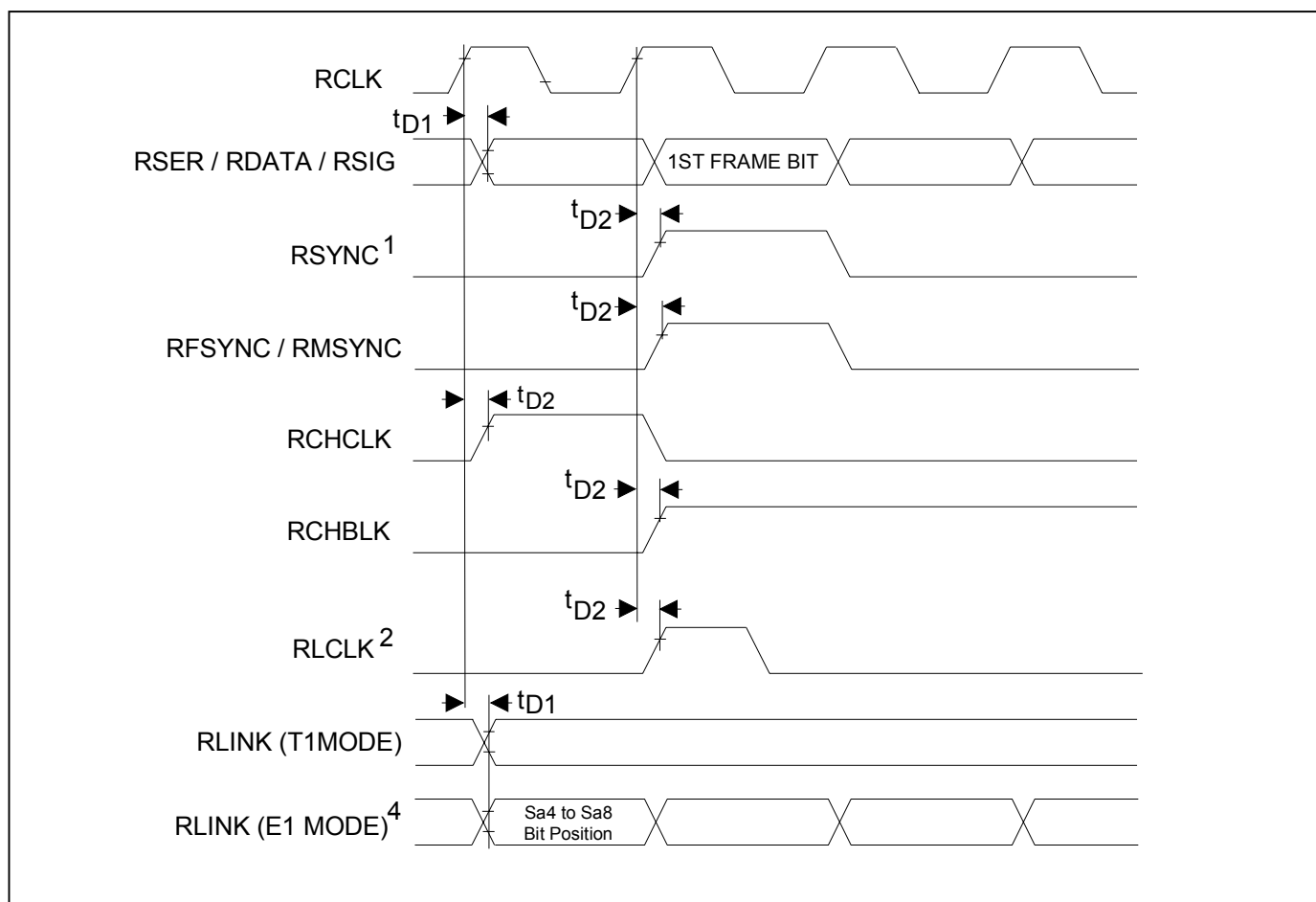
Figure 37-8. Receive-Side Timing
