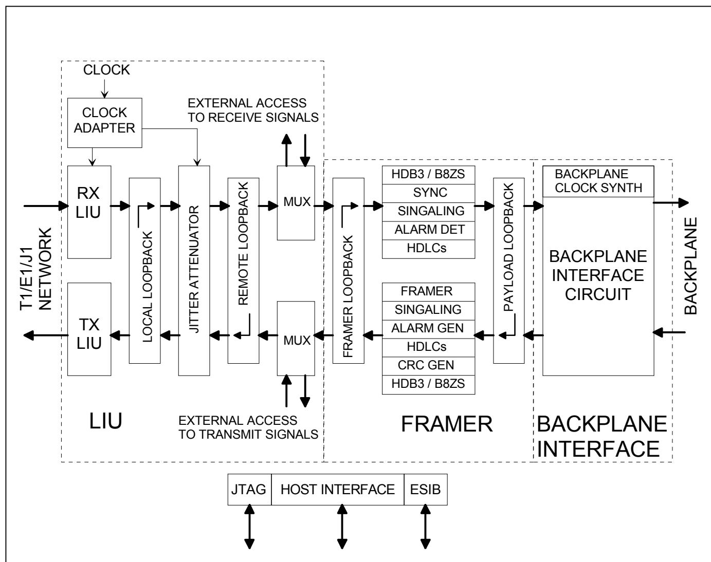
Figure 3-1. Block Diagram
