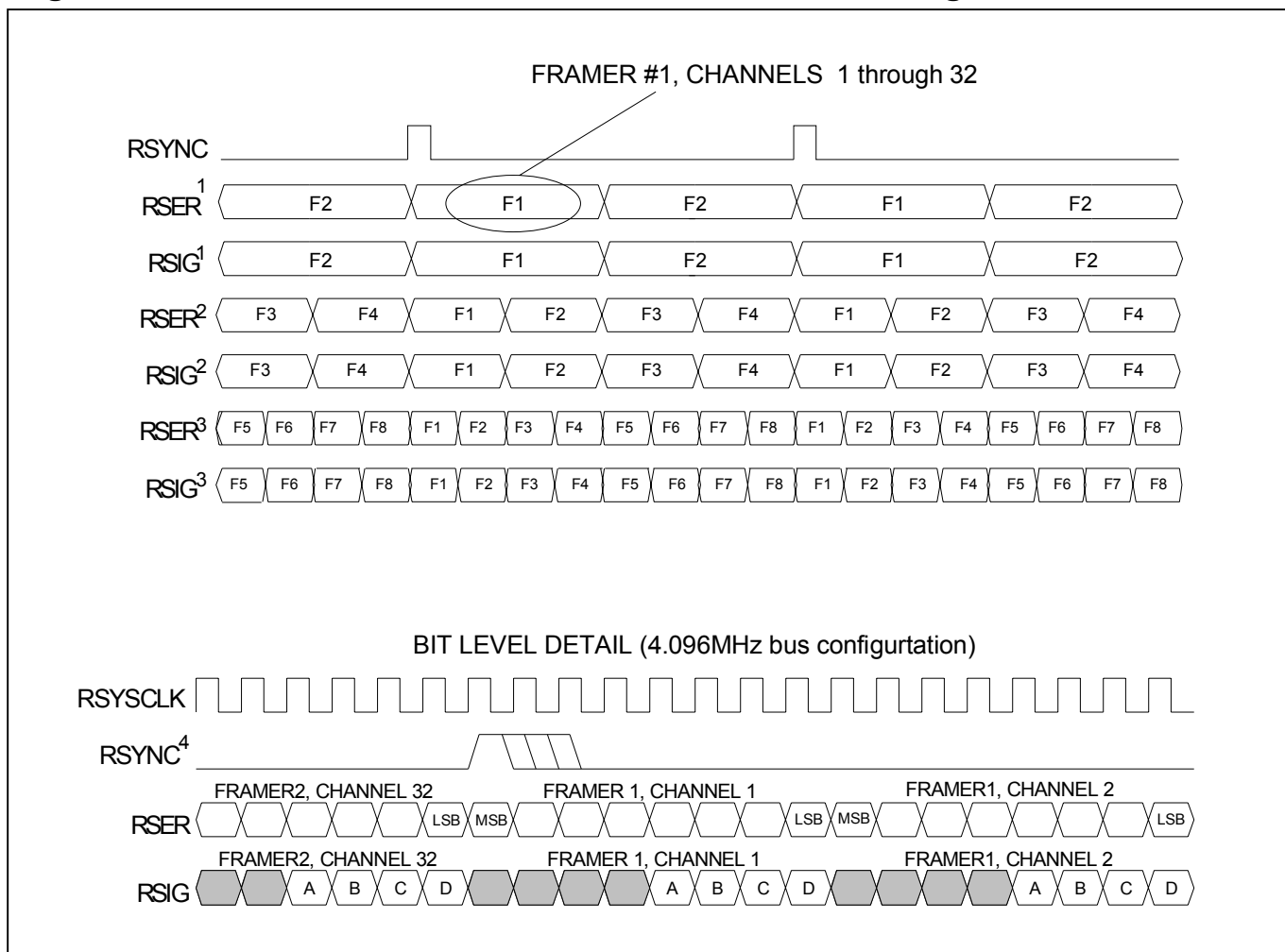
Figure 35-16. Receive IBO Frame Interleave Mode Timing
