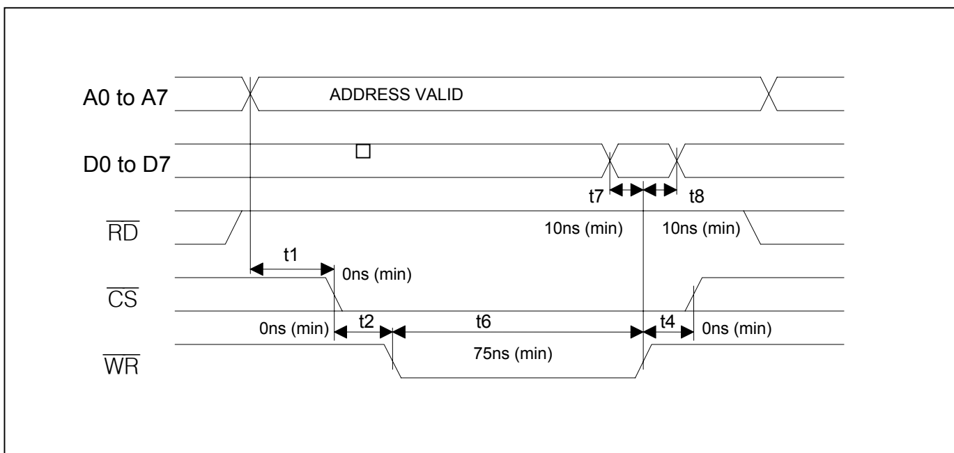
Figure 37-5. Intel Nonmultiplexed Bus Write Timing (BTS = 0/MUX = 0)
